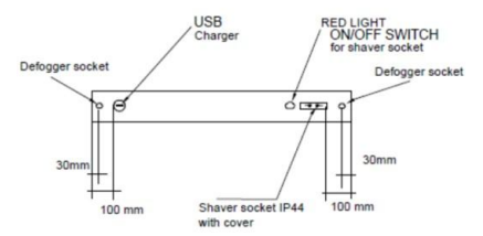
switch/socket/usb charger position detail
