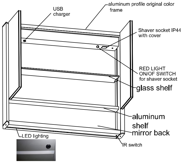
switch/socket/usb charger position detail
